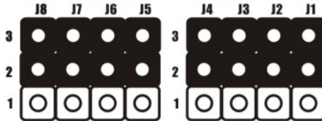
Jumper Settings(Default Mode:2-3 close)
