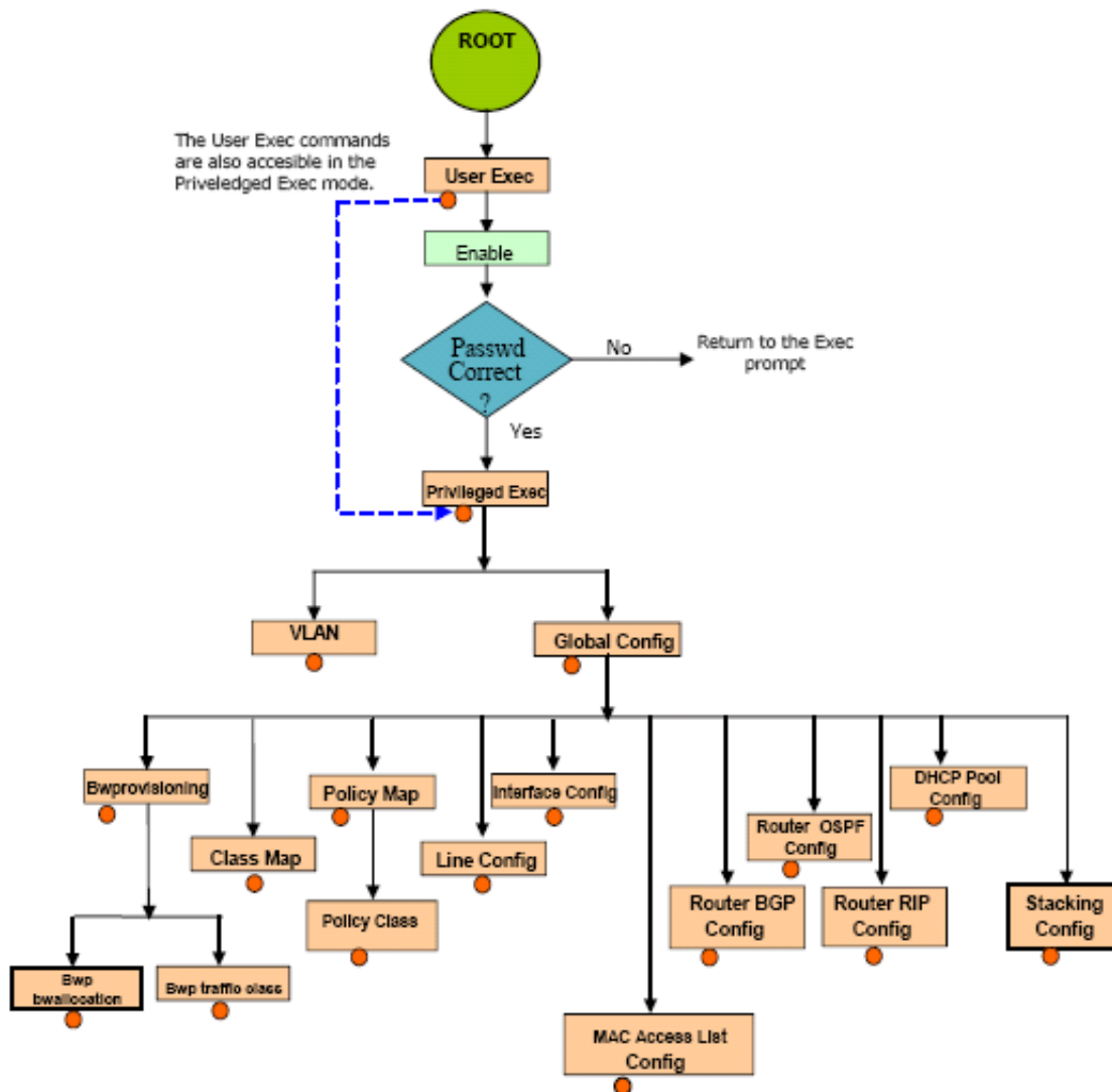
Figure 1. Mode-based CLI
