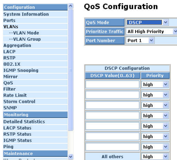
Fig. 4-23 DSCP Setting
