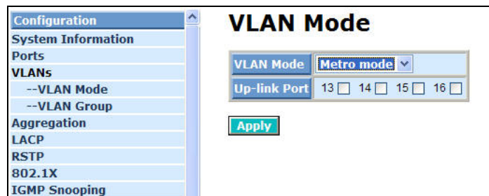
Fig. 4-6 Metro mode
