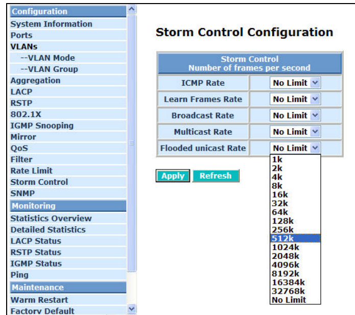
Fig.4-26 Storm Control Configuration
