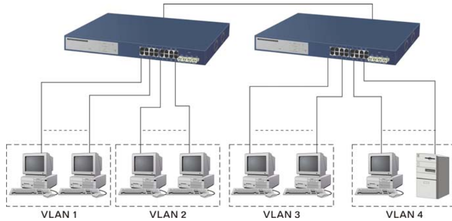
Fig. 2-4 Port-based VLAN Diagram
