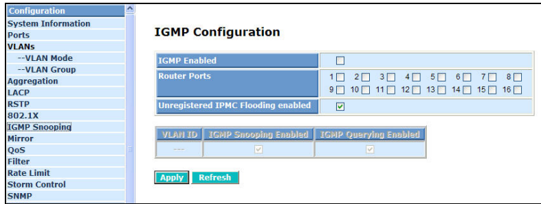
Fig. 4-19 IGMP Configuration
